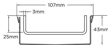
Profile 2
