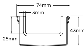
Profile 4
