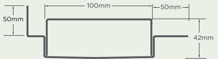
100mm TILE FLANGE
