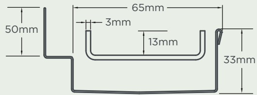
65mm TILE FLANGE With Tile Insert (Ti)
